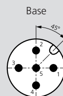
Male connector 5-pin M 12 x 1
