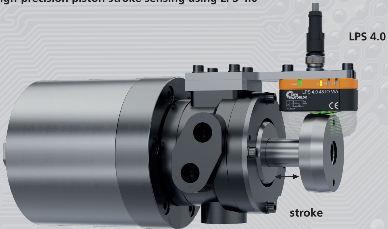
Clamping cylinder
