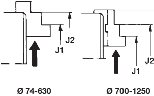
Internal chucking
