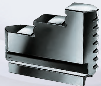
Reversible top jaw UB, hardened and ground
