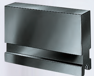
Unstepped jaw BL unstepped, soft, material 16MnCr5
