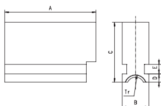
Garras blandas monoblock
