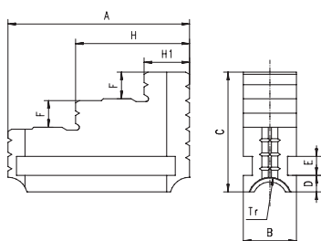
Garras monoblock reversibles
