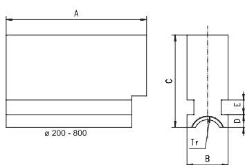
Garras blandas monoblock
